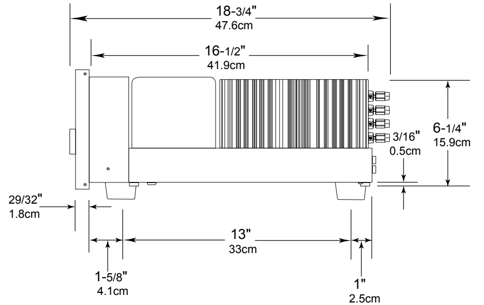
Side View of the MAC7200
